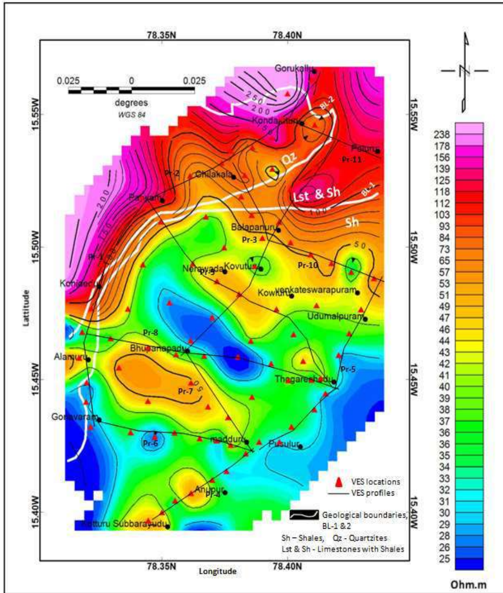
Figure 2. Contour map of apparent resistivity, AB/2=5m , of Panyam study area along with VES locations and profiles.
