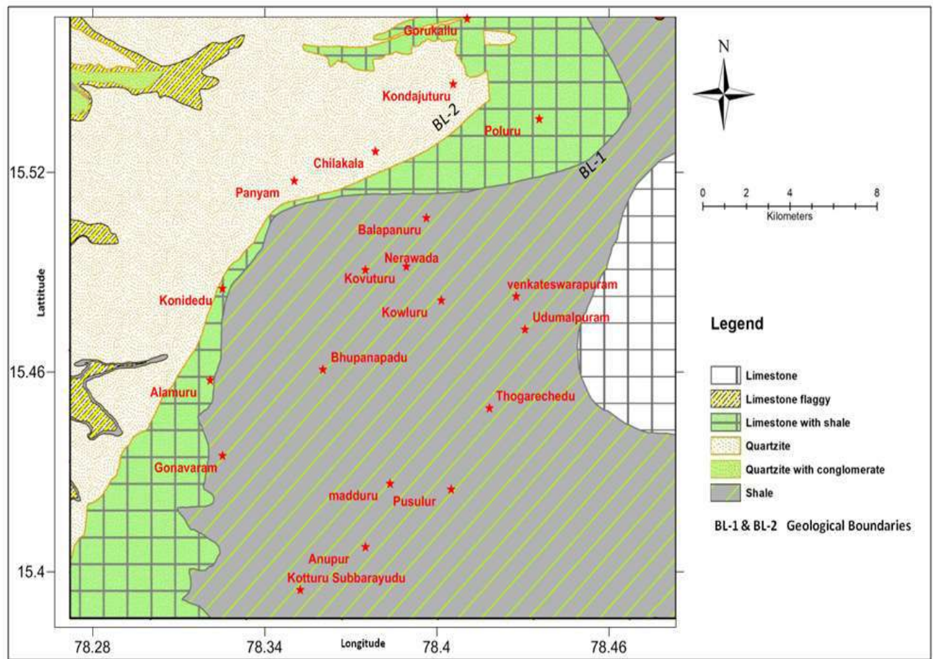
Figure1. Geological map of the Panyam mandal along boundary lines BL-1 and BL-2. (after GSI, 2005)
