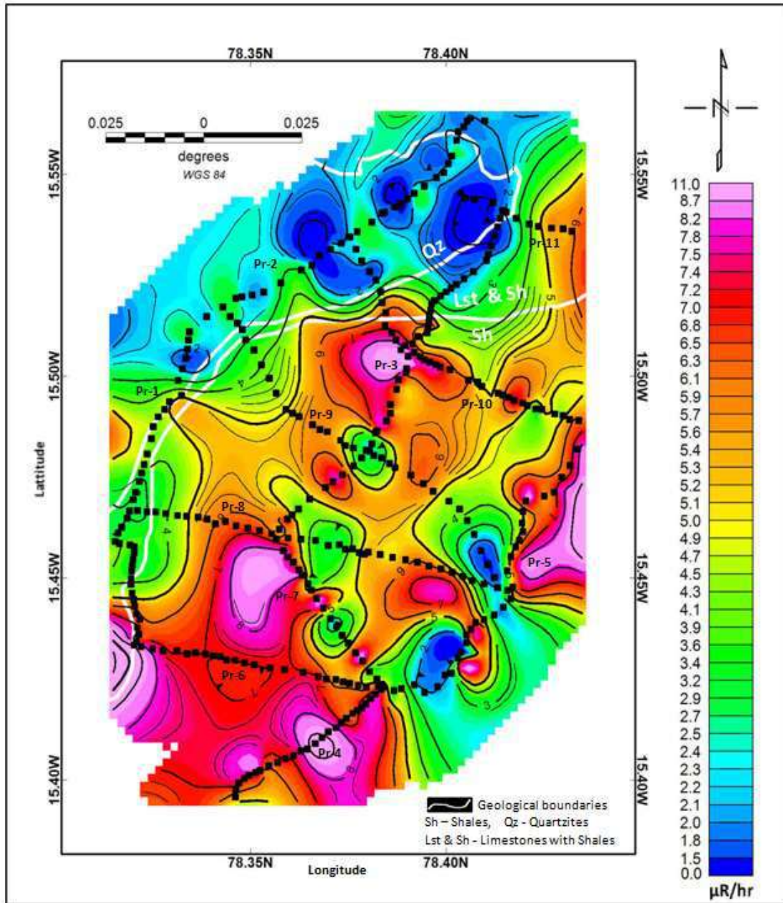
Figure 3. Radiometric contour map of Panyam mandal, along with radiometric profiles.
