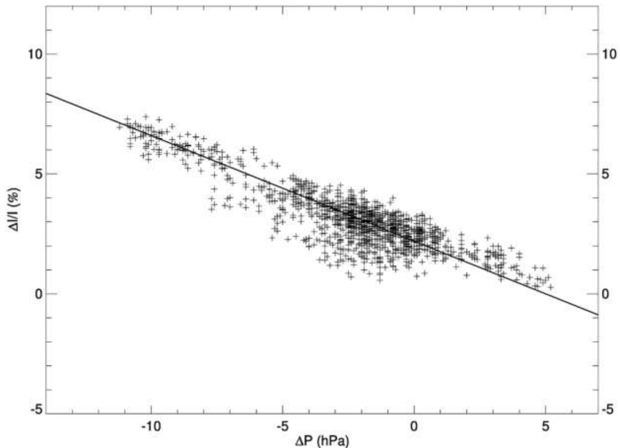
Figure 2. The autocorrelation between the pressure deviation and the relative cosmic ray intensity variation observed by the channel N12 of CARPET detector on July 2009. The black continuous line is given by Y = 2.2 - 0.44 * X and the correlation coefficient is 0.9.
