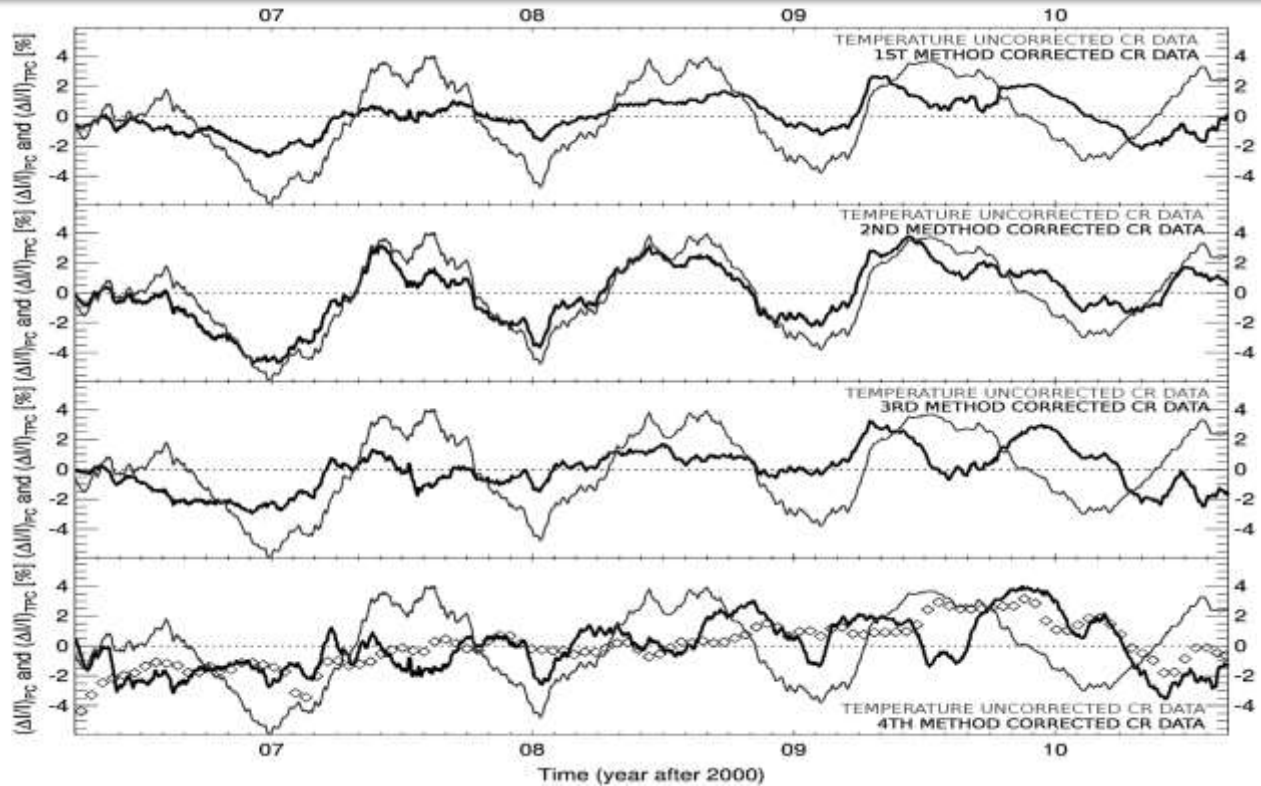
Figure 6. Monthly mean values of uncorrected by temperature cosmic ray intensity and of first, second, third, and fourth temperature methods corrected cosmic ray intensity observed by the CARPET detector between April 2006 and August 2010. The diamonds in the last panel represent the cosmic ray variation observed by the Moscow Neutron Monitor
