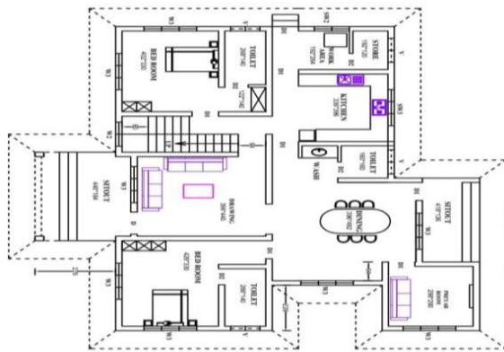
Fig 3. Ground floor plan of the building
