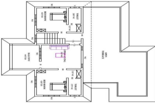
Fig 2. First-floor plan of the building
